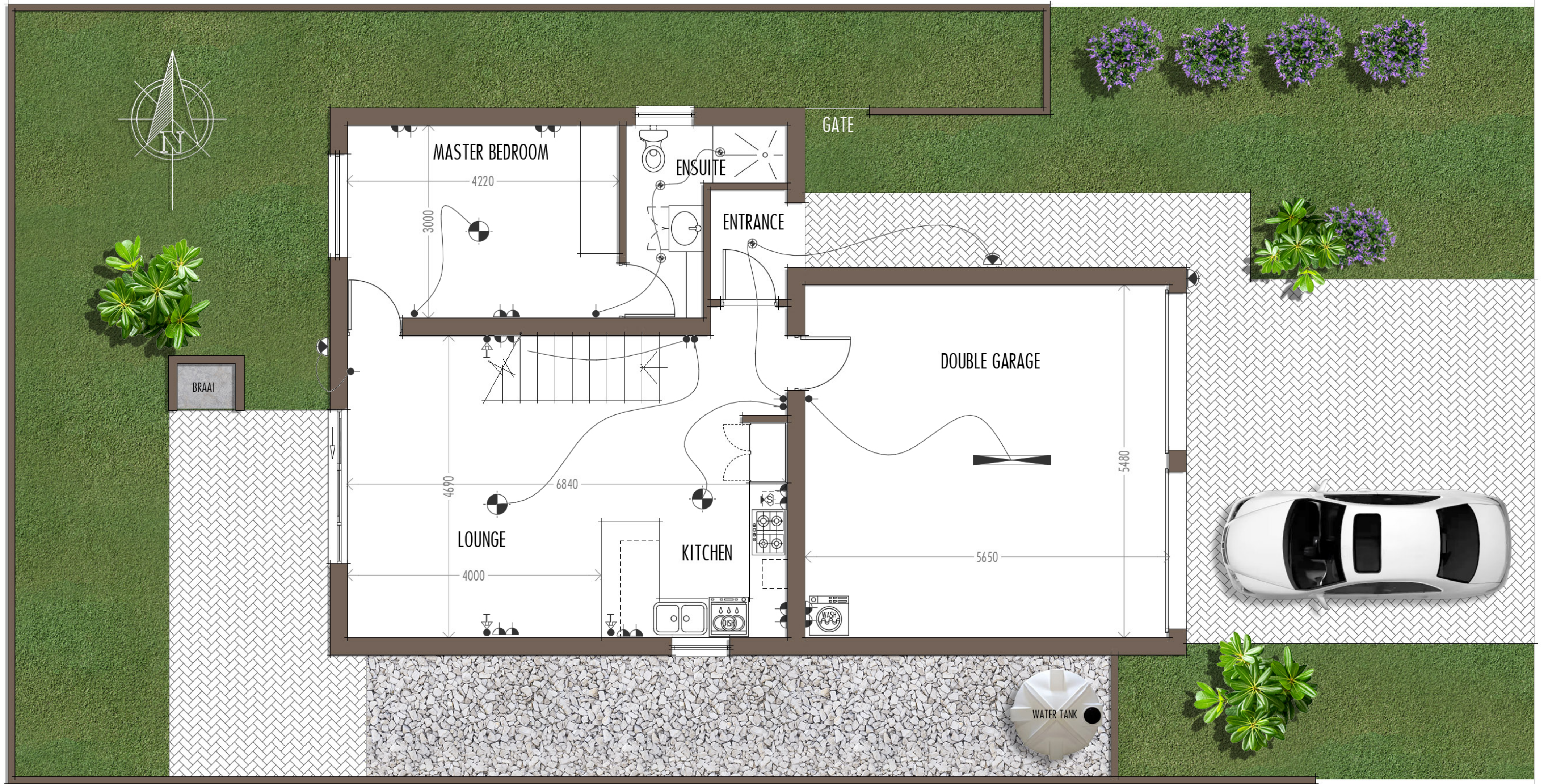
HOUSE NUMBER 04 - ERF 4692 - 137 m 2 GROUND FLOOR
