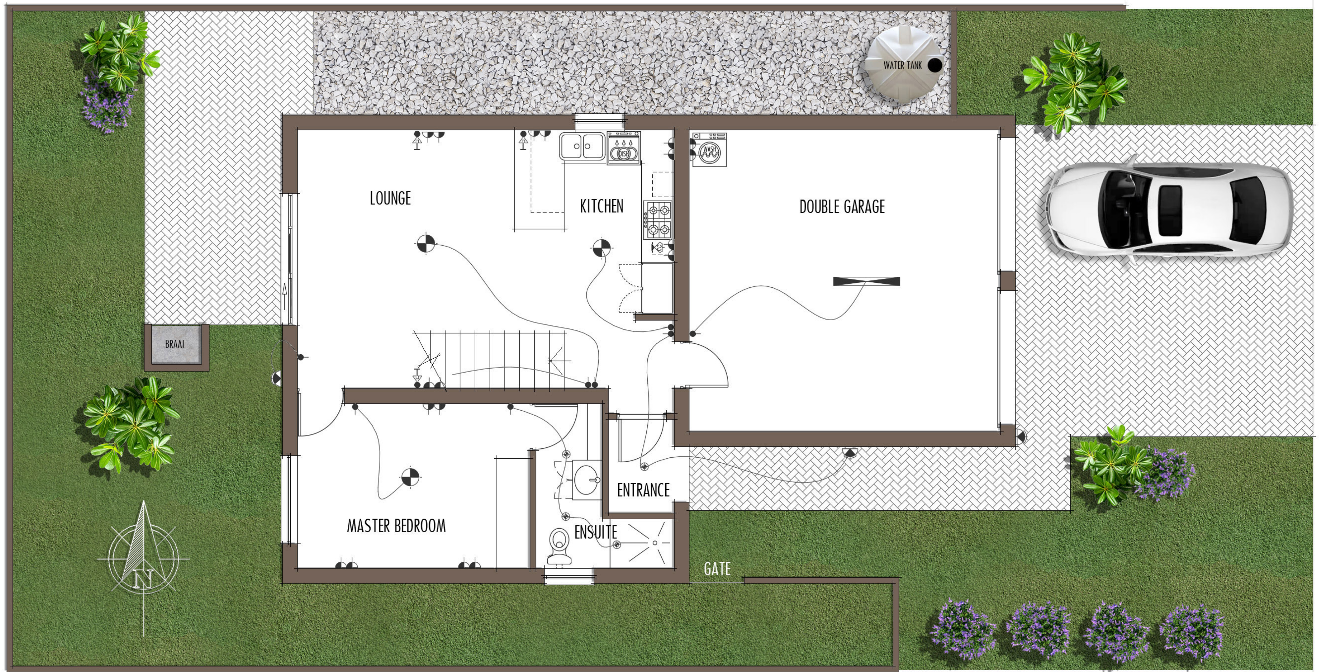
HOUSE NUMBER 07 - ERF 4693 - 137 m 2 GROUND FLOOR
